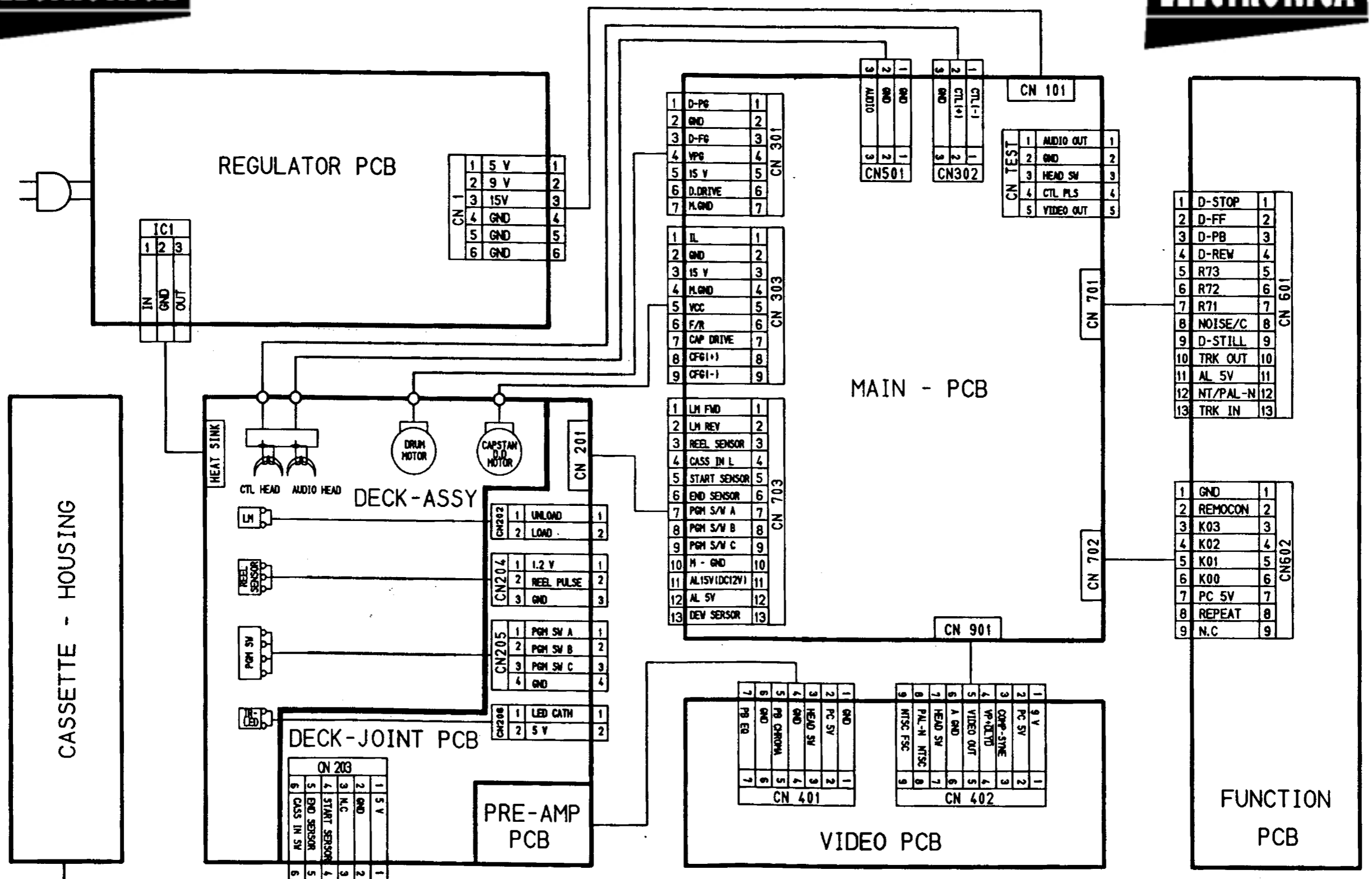
Total Wiring Diagram
